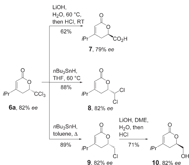
Scheme 3. Synthetic modification of the trichloromethyl group.
