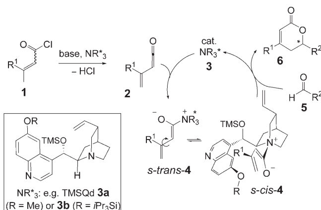
Scheme 1. Proposed [4+2] cycloaddition of \alpha,\beta -unsaturated acid chlorides 1 with aldehydes 5 providing lactones 6 .
