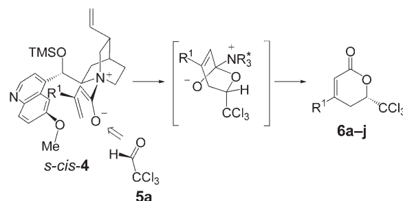
Scheme 2. Rationalization of the remote stereocontrol.
